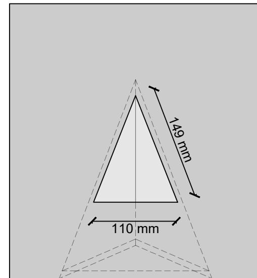
Back View Scale 1:5
